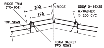
RIDGE DETAIL
